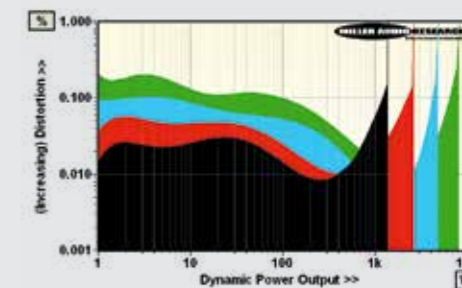
ABOVE: Dynamic power output versus distortion into 8ohm (black trace), 4ohm (red), 2ohm (blue) and 1ohm (green) speaker loads. Max. current is 91.1A
